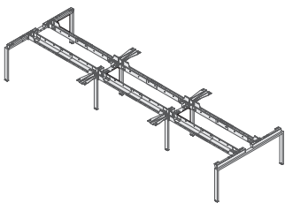
6-WAY DUAL BENCH BW4815 + [FINISH] 4800 (L) x 1500 (W) x 695 (H)
