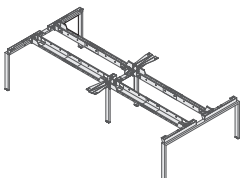
4-WAY DUAL BENCH BW3215 + [FINISH] 3200 (L) x 1500 (W) x 695 (H)
