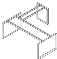
RECTANGULAR DESK LEG STRUCTURE INCL. L-EXTENSION DAL2010BLK 2000 (L) x 2000 (W) x 722 (H)
