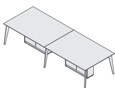
BOARDROOM - 3300 HT3312BLK 3300 (L) x 1200 (W) x 737 (H)
