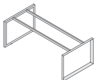
RECTANGULAR DESK LEG STRUCTURE DAL2000BLK 2000 (L) x 1000 (W) x 722 (H)
