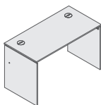
XPL113 + [FINISH] 1200 (L) x 600 (W) x 716 (H)
